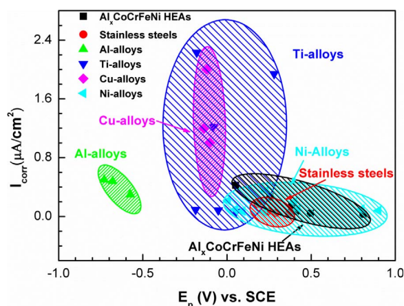
Fig. 11. Comparison of corrosion properties between HEAs and conventional alloys [60–66] in the 3.5 wt.% NaCl solution. The higher pitting potential ( E_p ) and lower corrosion-current density ( I_{corr} ) of Al_xCoCrFeNi HEAs indicate that the localized and general corrosion-resistant properties of the Al_xCoCrFeNi HEAs are comparable or even superior to that of conventional corrosion-resistant alloys.
