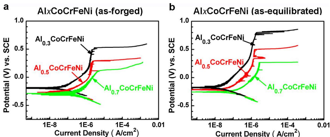
Fig. 7. Potentiodynamic polarization curves of the as-forged (a) and as-equilibrated (b) \text{Al}_x\text{CoCrFeNi} ( x = 0.3, 0.5 , and 0.7 ) alloys, performed with the scan rate of 100 \text{ mV/min} in the 3.5 \text{ wt.}\% NaCl solution at room temperature.
